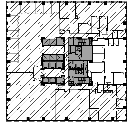
2 KEY PLAN 1/64" = 1'-0"
