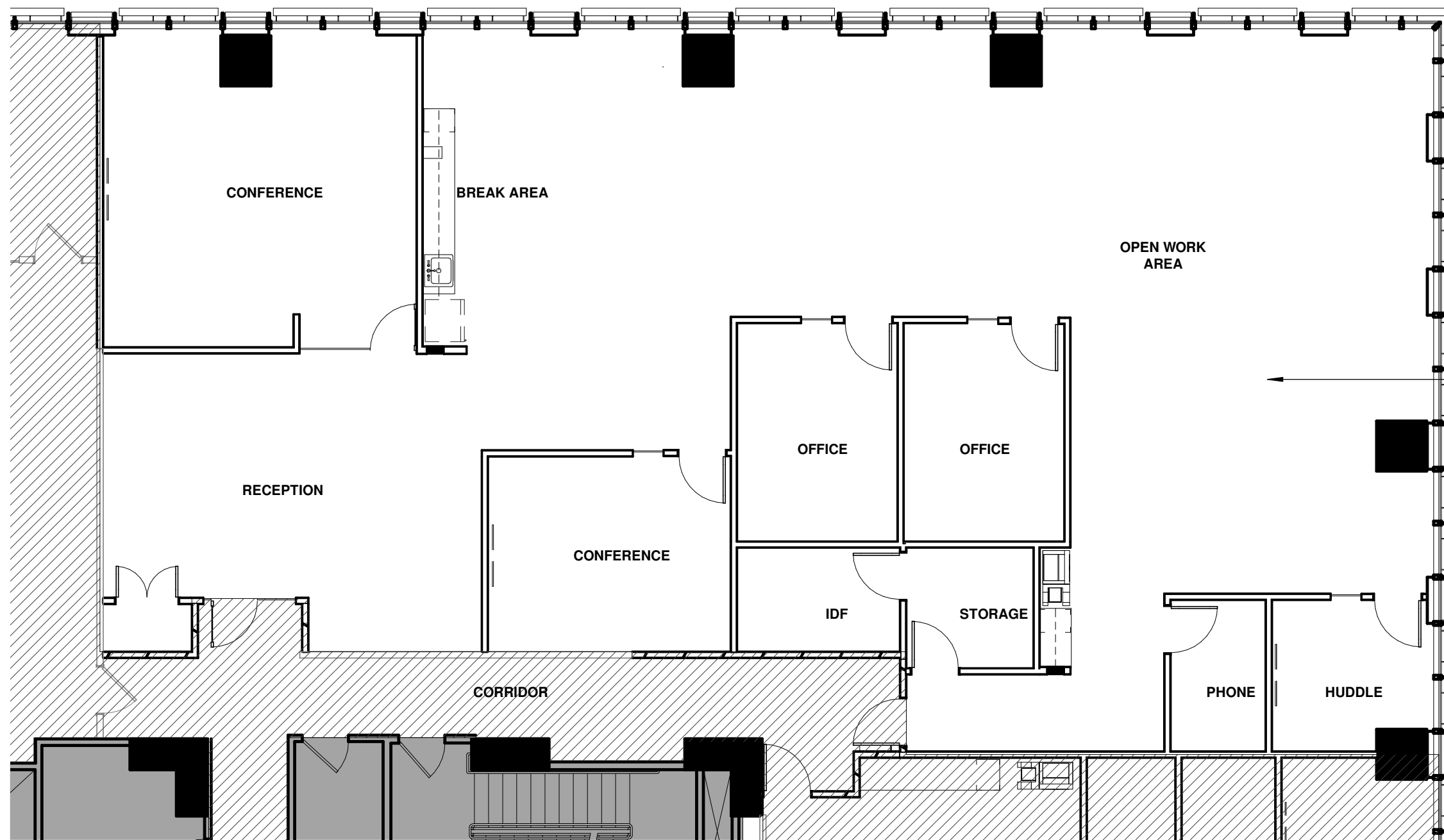
1 Level 5- Marketing Suite B 1/8" = 1'-0"
