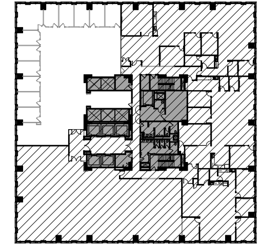
1 Suite A - KEY PLAN 1/64" = 1'-0"
